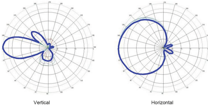
E-field elevation & Azimuth Patterns
